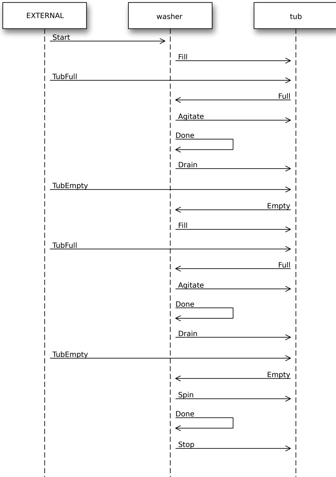
Figure 8: Example Sequence Diagram
